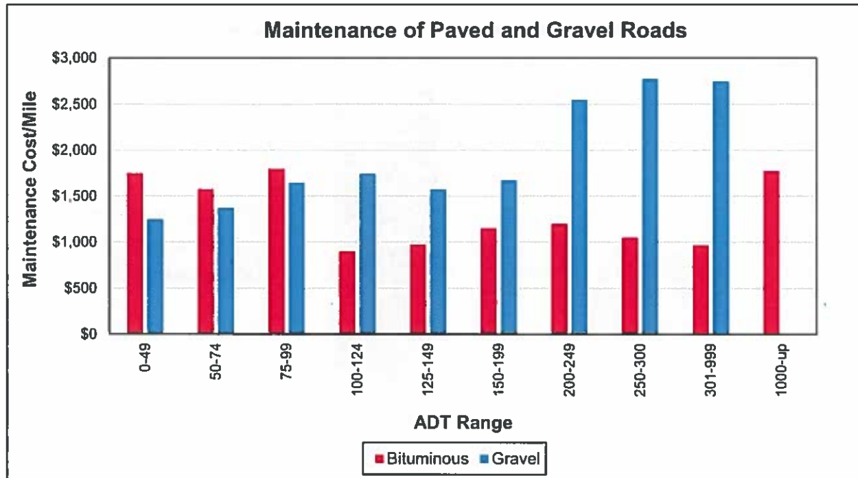
Figure 13: Economics of Upgrading an Aggregate Road (The Minnesota Local Road Research Board, 2005)
