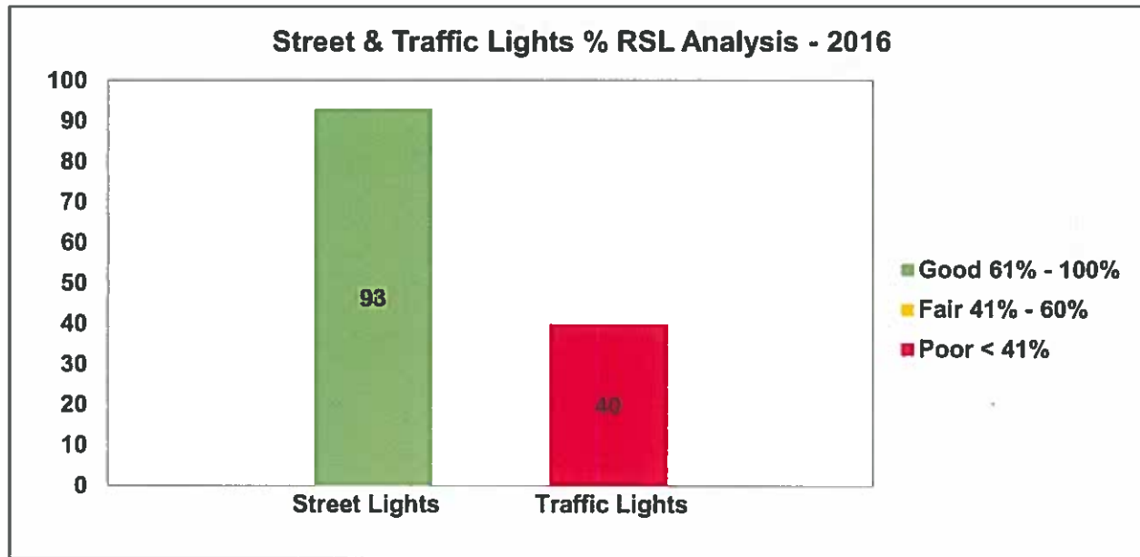
Figure 22: Street & Traffic Lights Condition Rating
