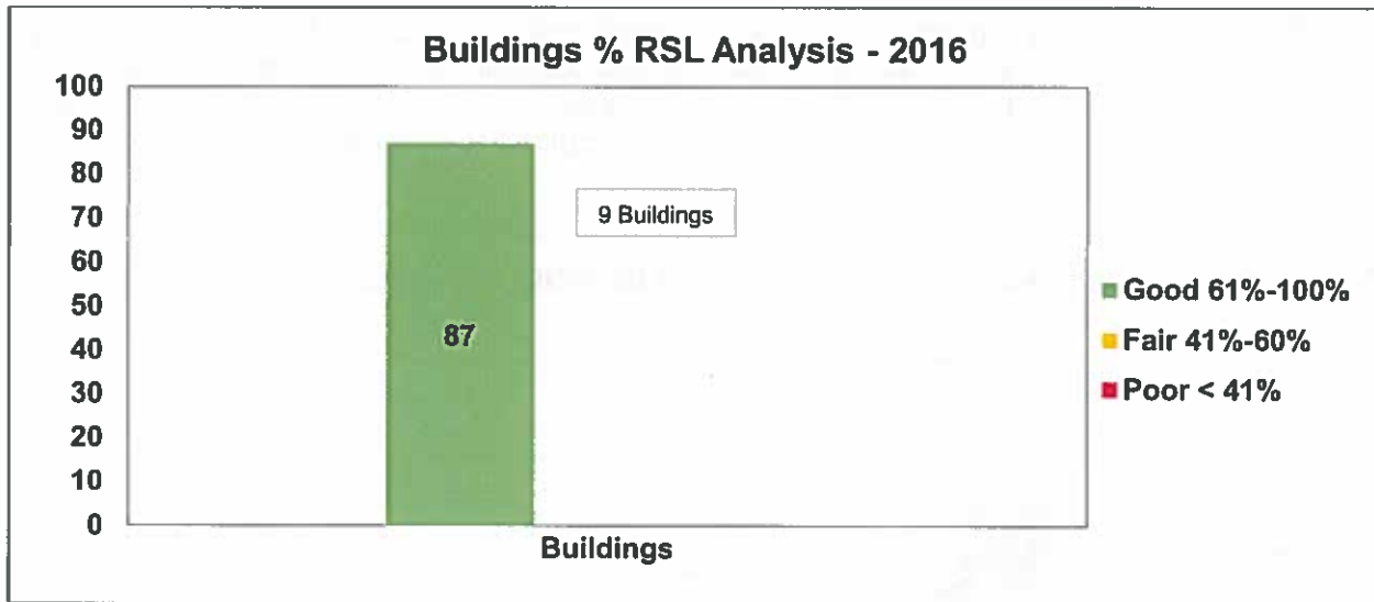
Figure 19: Buildings Condition Rating
