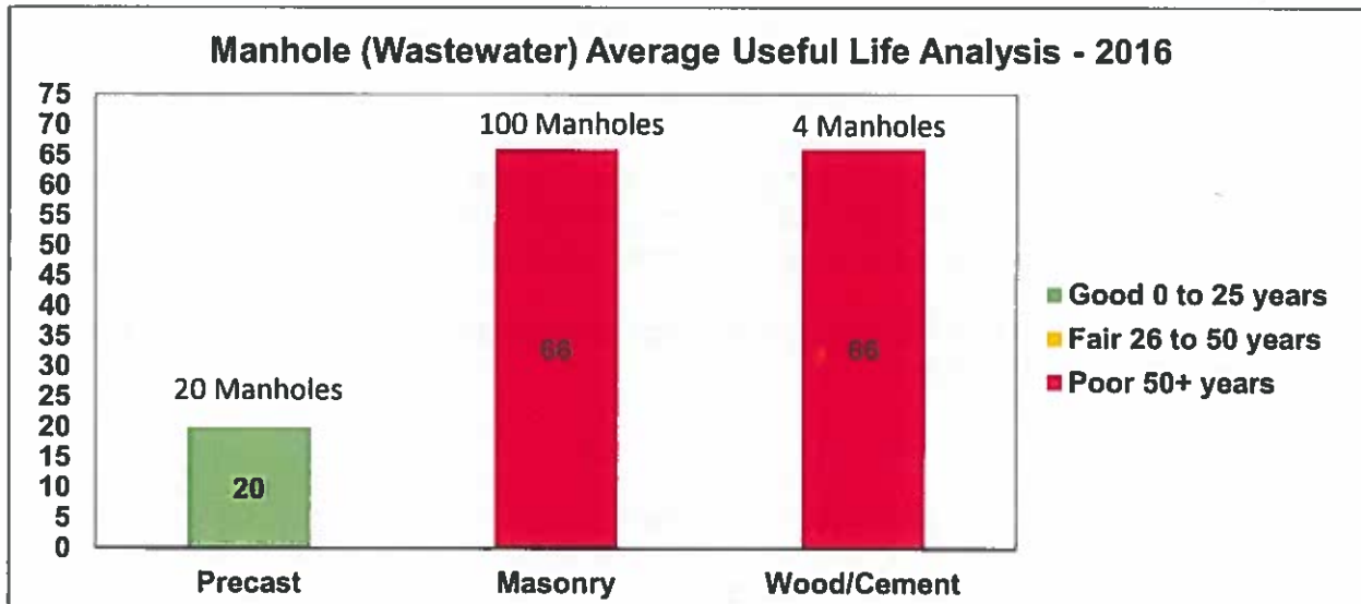
Figure 31: Manholes (Wastewater) Condition Rating
